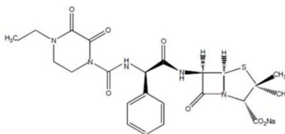
Piperacillin sodium
